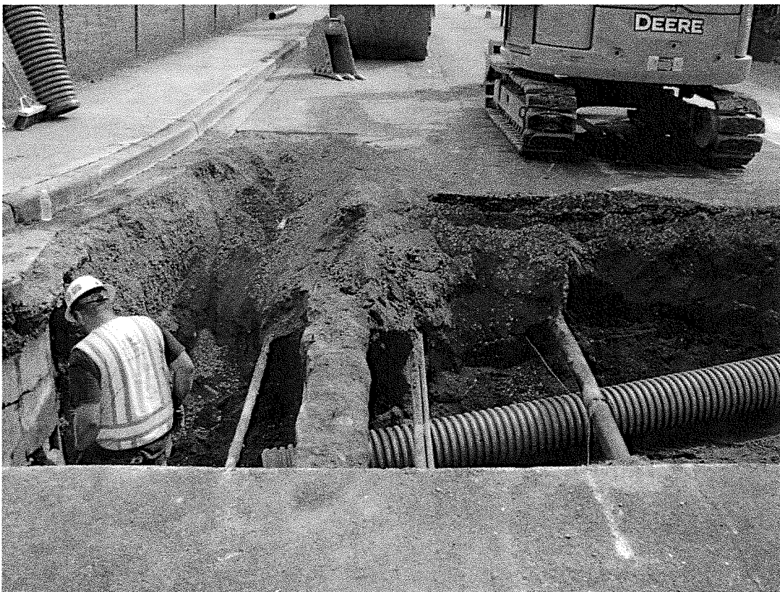
Installation of a stormwater pipe across Roberts Drive at Bruckners Way
